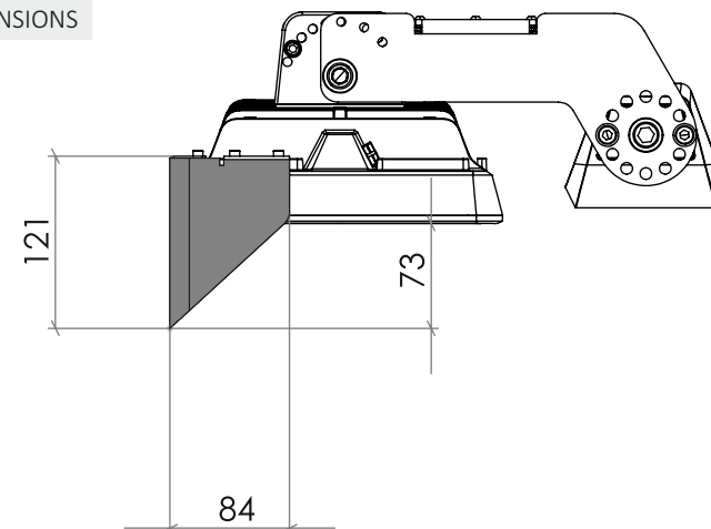
CANOPY DIMENSIONS
