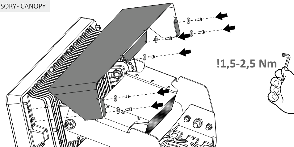
ACCESSORY- CANOPY
