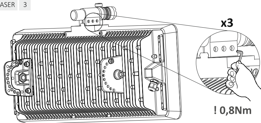
ACCESSORY- LASER 3
